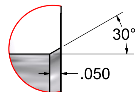
DETAIL A TYPICAL O-RING LEAD IN
