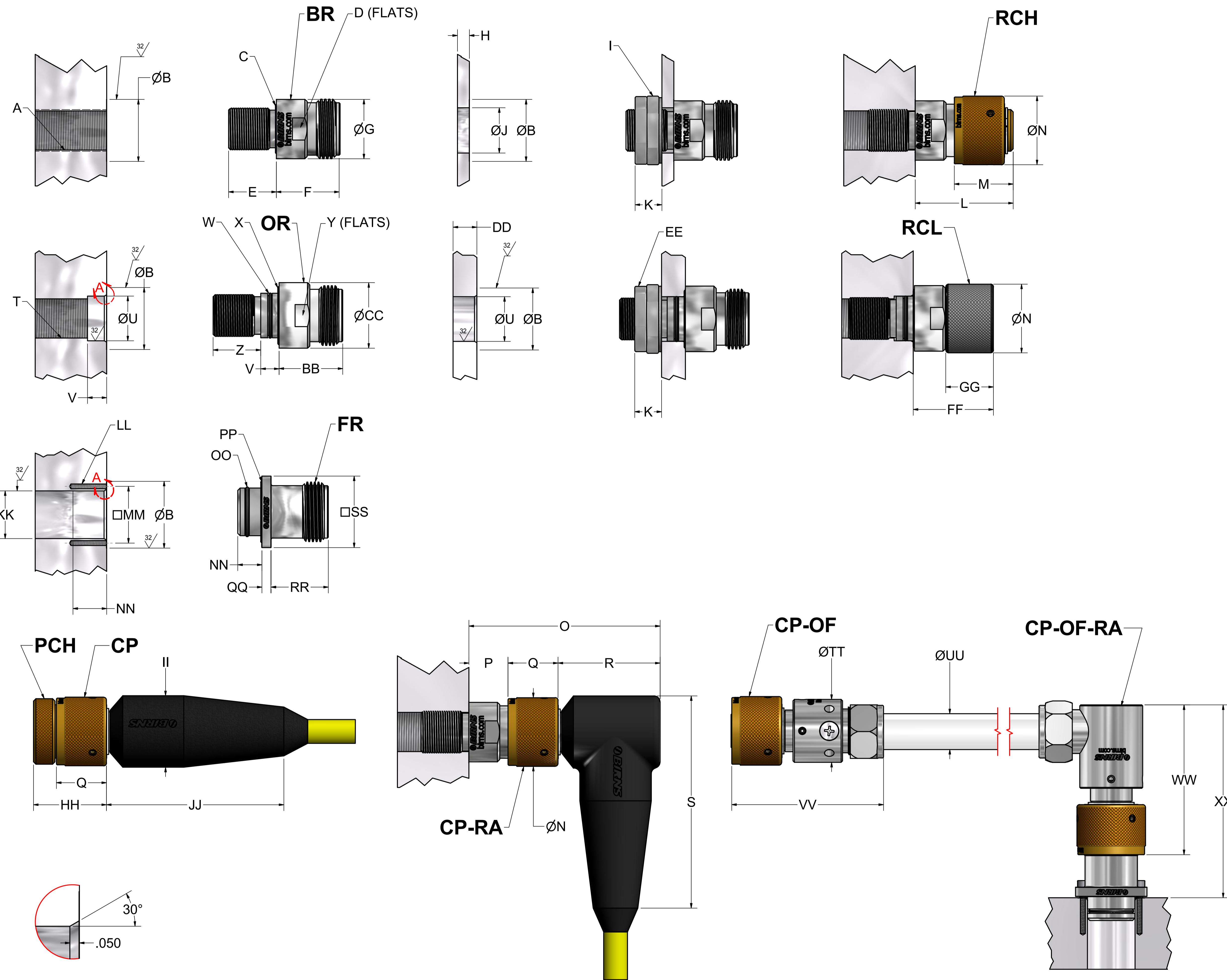
DETAIL A TYPICAL O-RING LEAD IN
